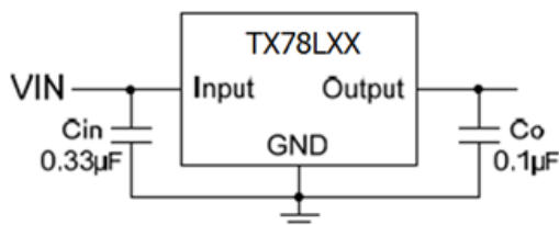
Fig.1 Typical Application
