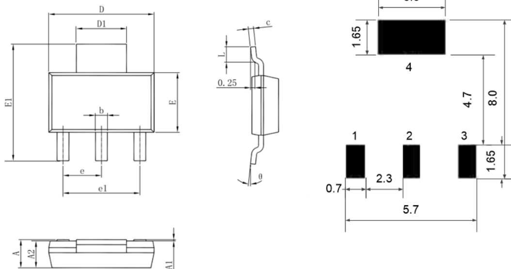
SOT-223 PACKAGE OUTLINE DIMENSIONS
