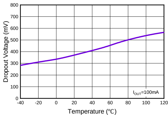
(9) Dropout Voltage VS Temperature
